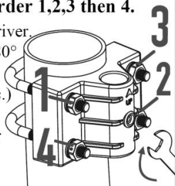
Figure 6: Sensor package mounting diagram 6-4
