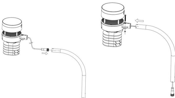
Figure 4: Sensor package mounting diagram 6-2
